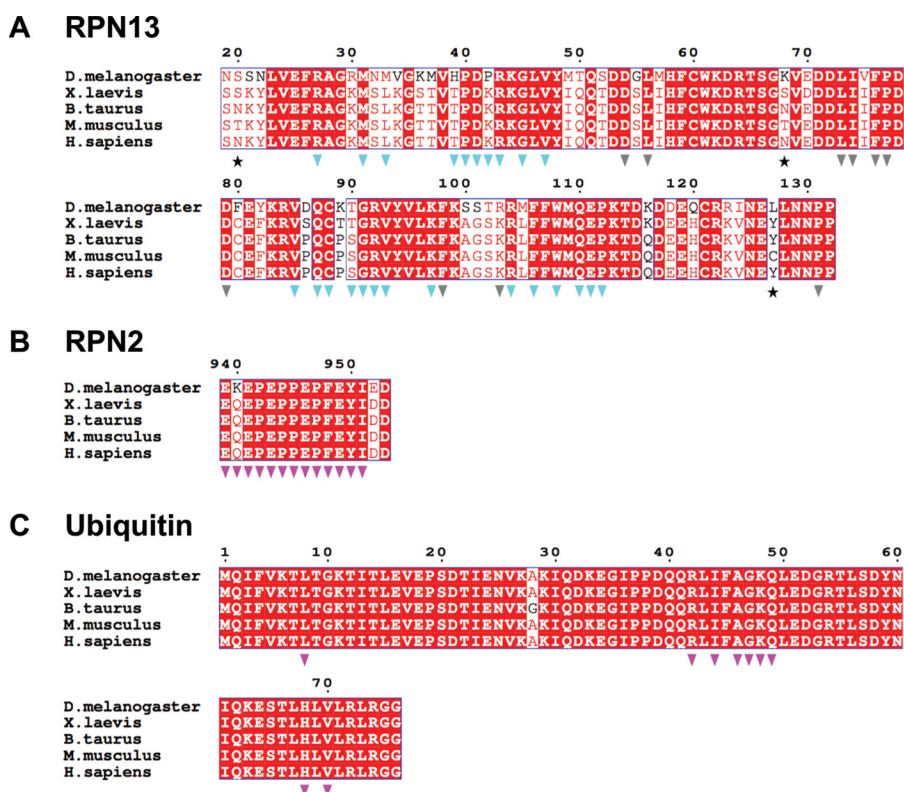
Figure 3. Sequence alignments of RPN13, RPN2, and ubiquitin from higher eukaryotes. A, RPN13 alignments. Stars indicate residues not conserved between mouse and human. Blue triangles indicate residues at the RPN13-RPN2 interface. Gray triangles indicate residues at the RPN13-ubiquitin interface. B, RPN2 sequence alignment. Magenta triangles indicate residues at the RPN13-RPN2 interface. C, ubiquitin sequence alignment; magenta triangles indicate residues at the RPN13-ubiquitin interface.
